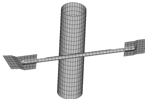
BOLT ANALYSIS BY A. TABIEI Time = 0
