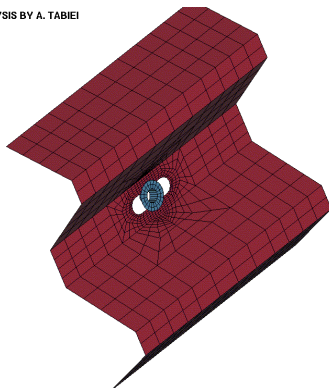
BOLT ANALYSIS BY A. TABIEI Time = 0
